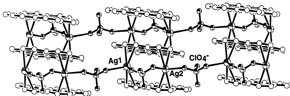
Fig. 8. Triple-layer polymeric structure of [\text{Ag}_4(\text{L}^5)_3(\text{ClO}_4)_4] ( 31 ).
