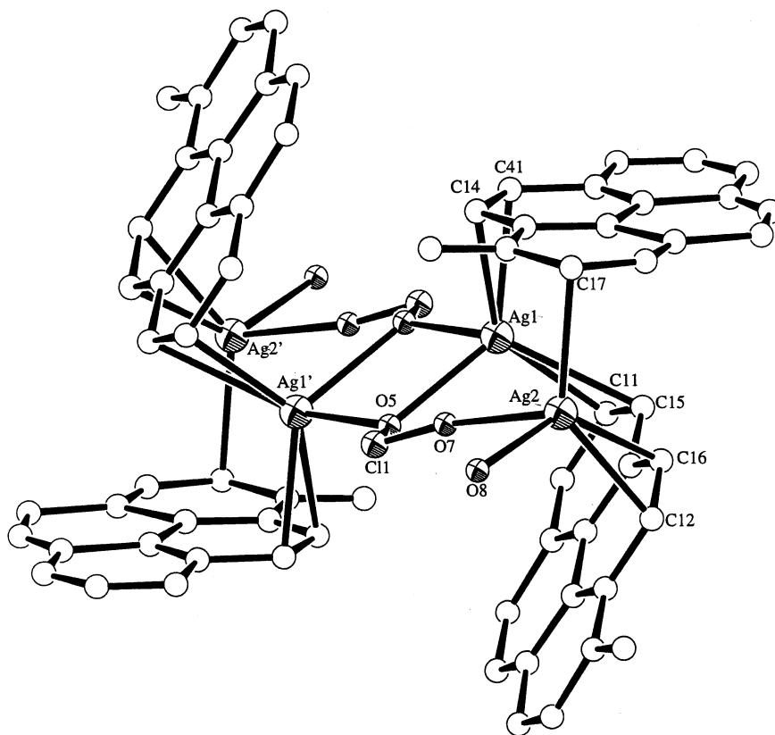
Fig. 4. Sandwich tetrameric structure of [\text{Ag}(\text{L}^2)\text{ClO}_4]_4 ( 27 ). The non-coordinating oxygen atoms of the perchlorate ions are omitted.
